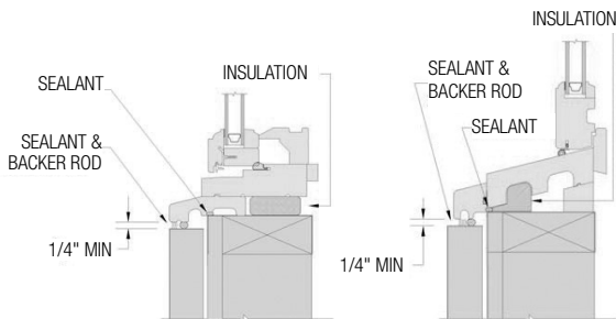
FIG. 17: CASEMENT SILL
