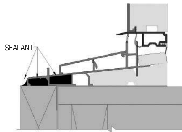
FIG. 19: IN-SWING SILL
