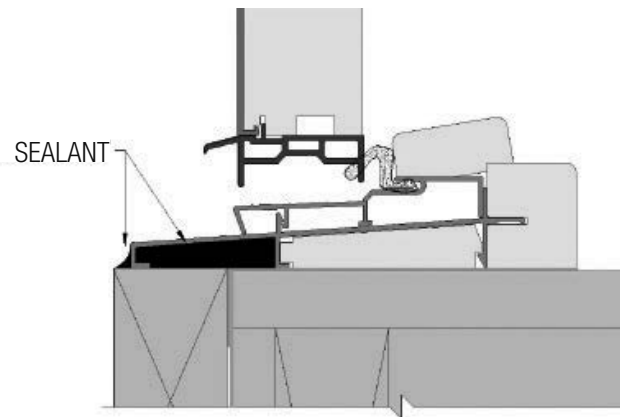
FIG. 18: OUT-SWING SILL
