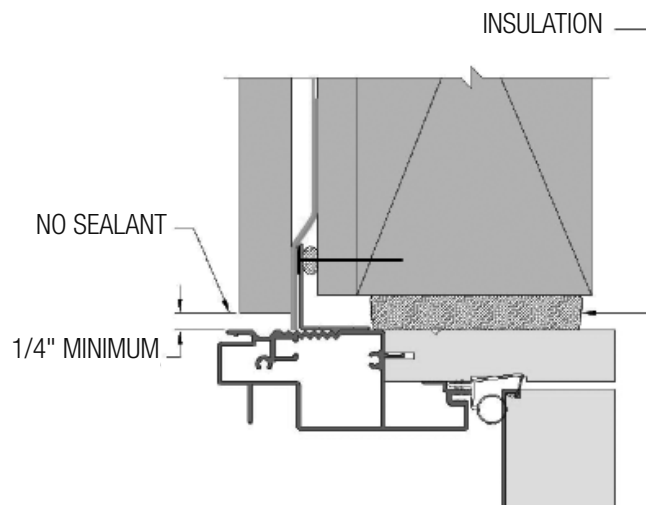
FIG. 26: IN-SWING HEAD JAMB
