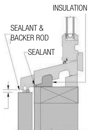
FIG. 18: DOUBLE HUNG SILL
