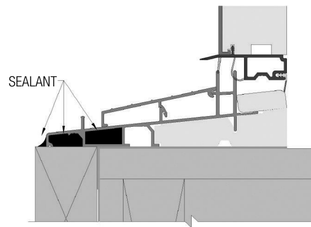
FIG. 19: IN-SWING SILL
