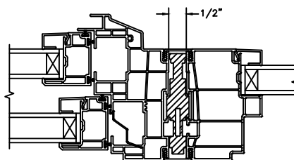
VERTICAL 1/2" MULLION OPERATOR/FIXED
