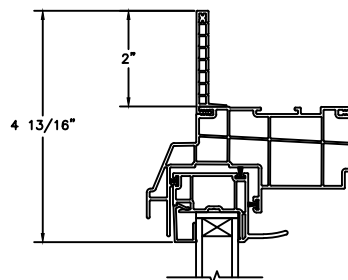
2" FLANGE
