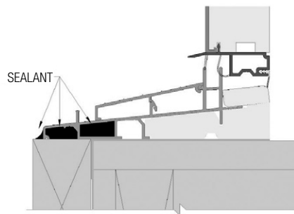
FIG. 19: IN-SWING SILL
