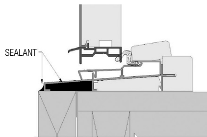
FIG. 18: OUT-SWING SILL
