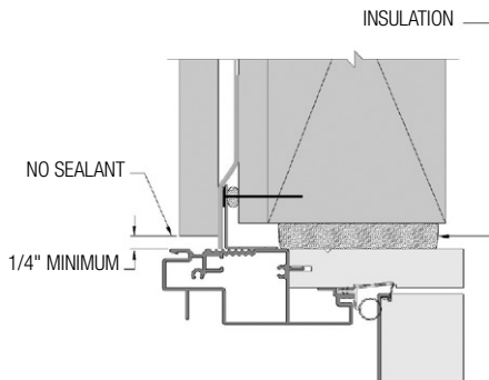
FIG. 26: IN-SWING HEAD JAMB
