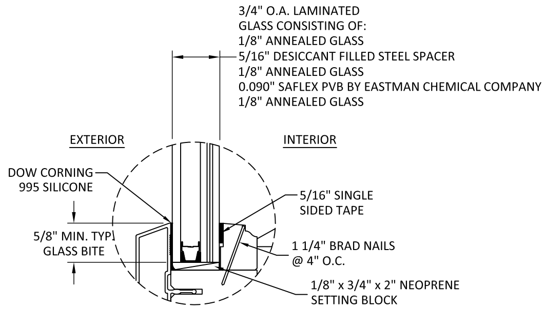
GLAZING DETAIL
