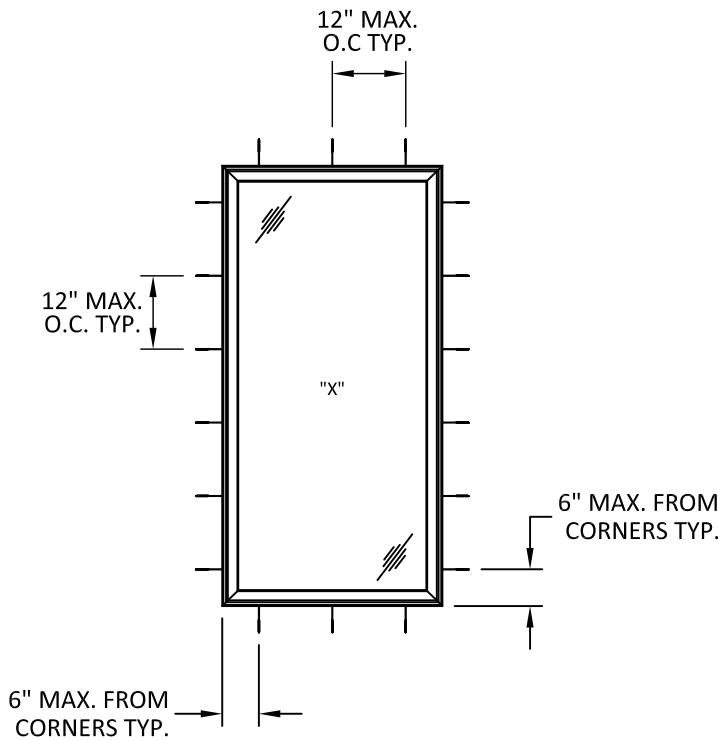
ANCHOR LAYOUT CLIP OR THROUGH FRAME INSTALLATION
