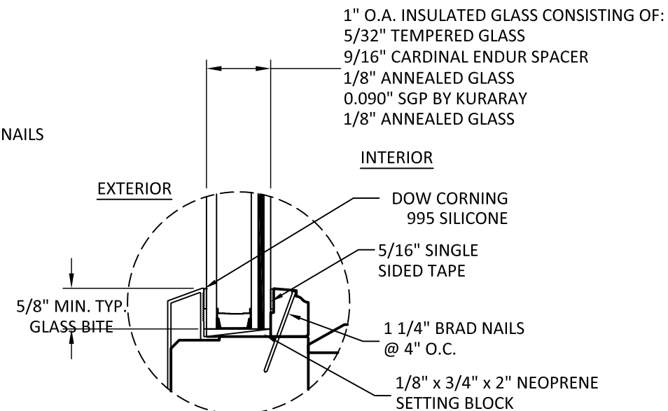
GLAZING DETAIL 4
