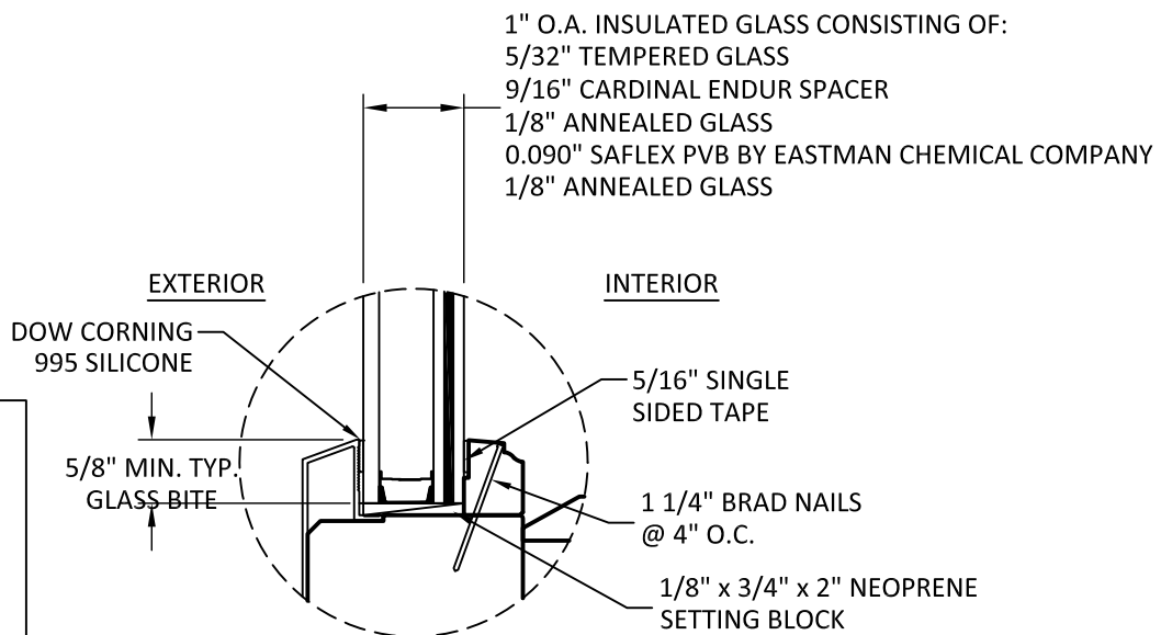
GLAZING DETAIL 2
