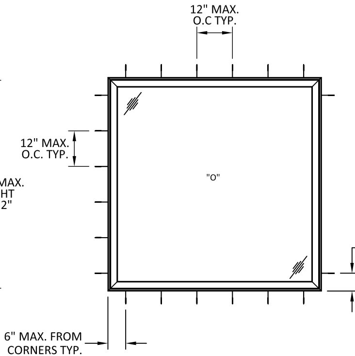
ANCHOR LAYOUT CLIP OR THROUGH FRAME INSTALLATION
