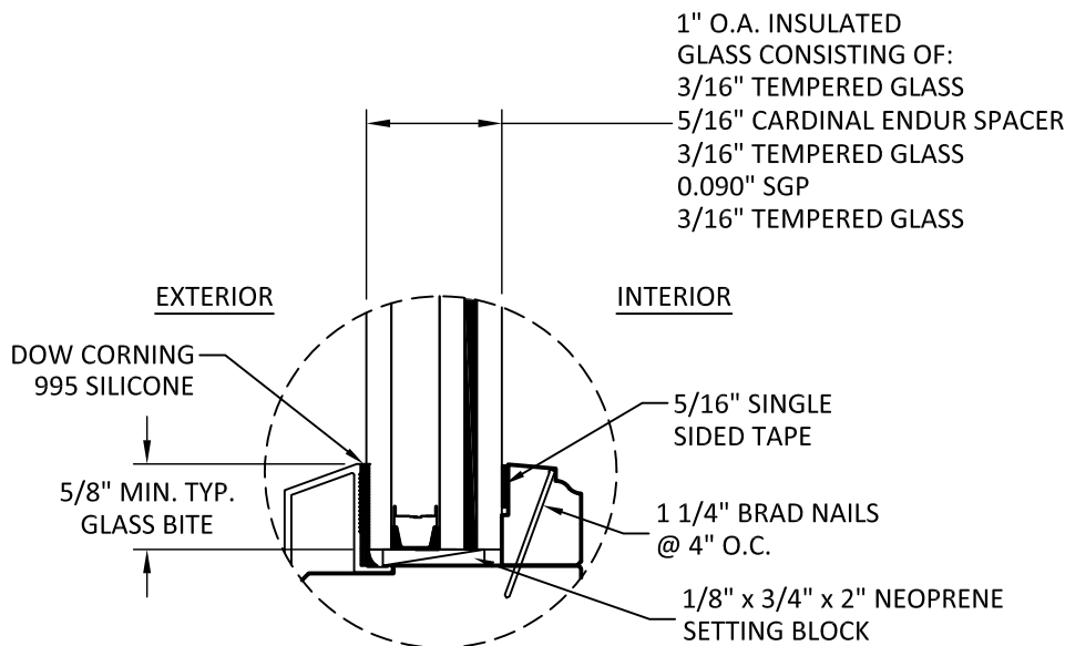
GLAZING DETAIL G1
