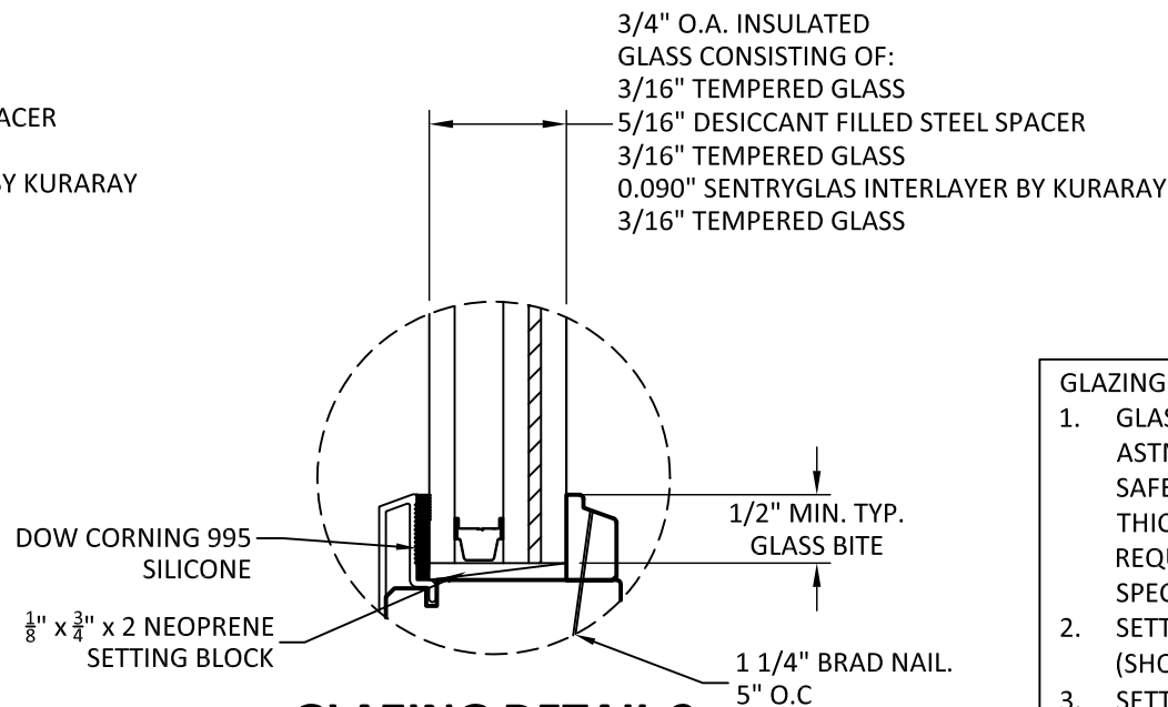
GLAZING DETAIL 2
