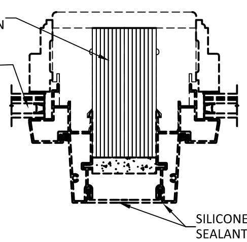
C 2 DUAL DIRECT SET VERTICAL MULLION
