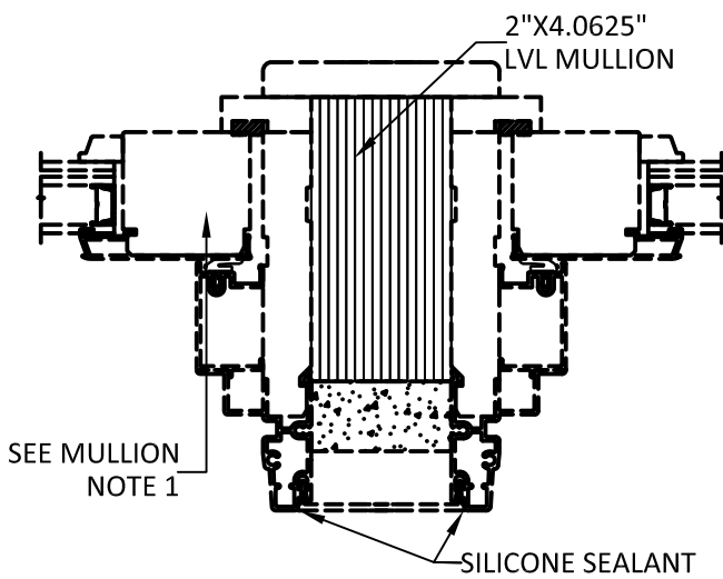
A 2 DUAL DOUBLE HUNG PIC. VERTICAL MULLION
