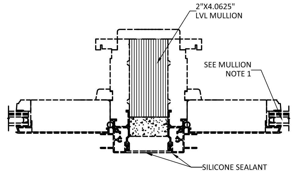
H 2 DUAL SLIDING PATIO VERTICAL MULLION
