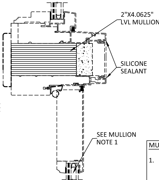
O 3 OUTSWING-CASEMENT OP HORIZONTAL MULLION
