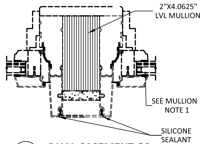
E 2 DUAL CASEMENT OP. VERTICAL MULLION
