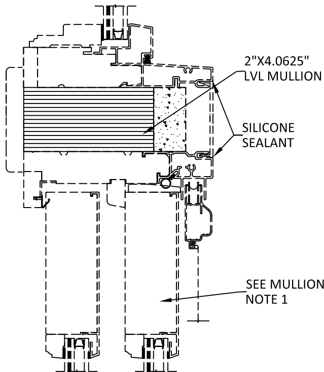
M 3 SLIDING - DIRECT SET HORIZONTAL MULLION
