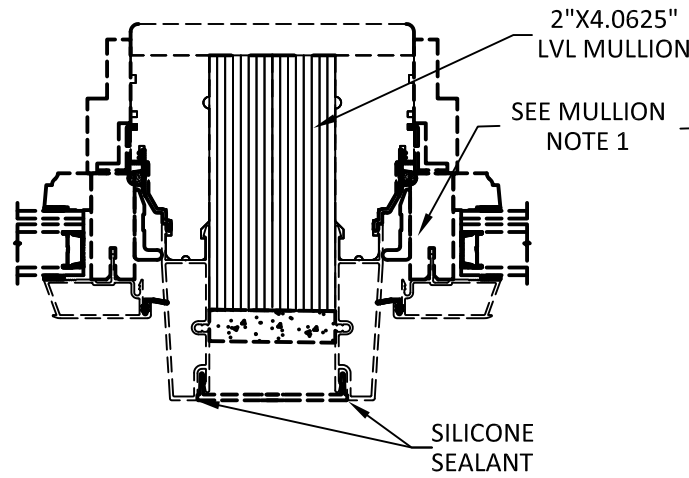
B 2 DUAL CASEMENT PICTURE VERTICAL MULLION
