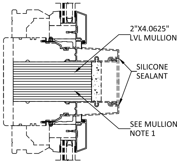
J 3 DUAL CASEMENT PIC HORIZONTAL MULLION
