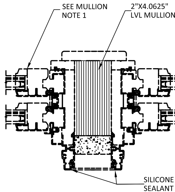
G 2 DUAL DOUBLE HUNG OP. VERTICAL MULLION
