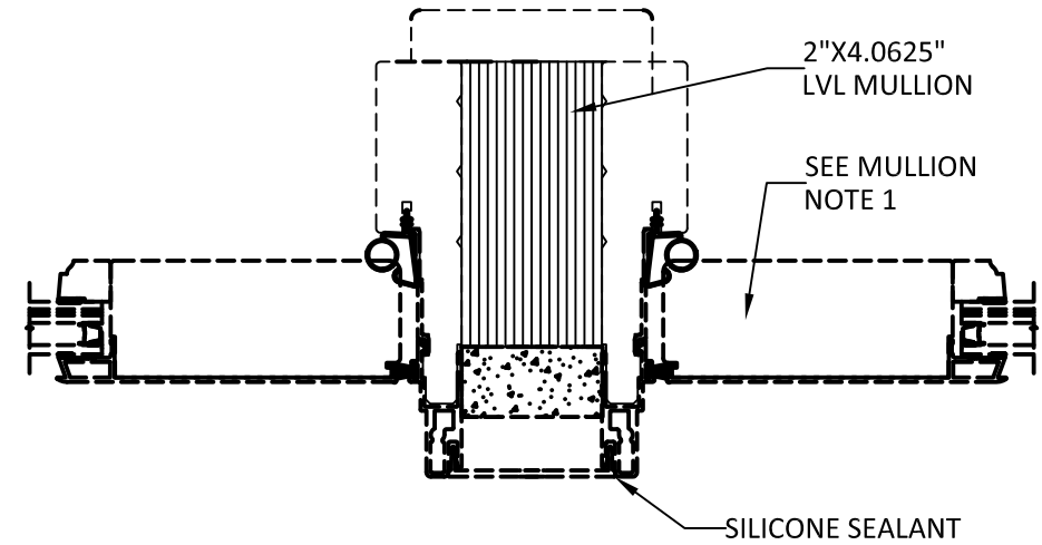
D 2 DUAL OUTSWING PATIO VERTICAL MULLION
