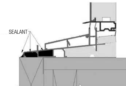
FIG. 18: IN-SWING SILL
