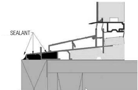
FIG. 18: IN-SWING SILL
