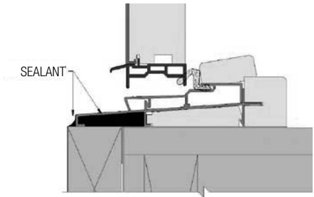
FIG. 17: OUT-SWING SILL
