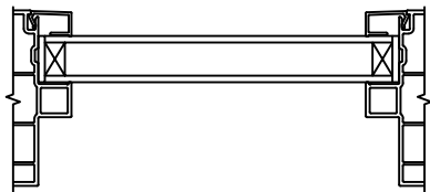
INSULATING GLASS
