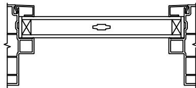
3/4" PROFILED INNERGRILLE
