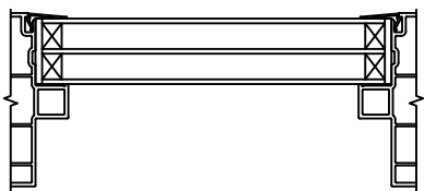
TRIPLE IG INSULATING GLASS
