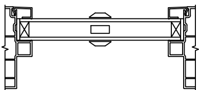
7/8" GRILLE BAR WITH INNERBAR
