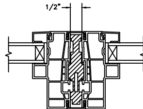
VERTICAL 1/2" MULLION RADIUS/RADIUS
