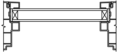
INSULATING GLASS
