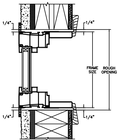
HEAD JAMB & SILL 2 X 4 FRAME WITH STUCCO 1" OR 2" FLANGE OPTION
