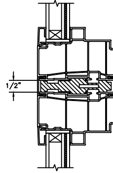
HORIZONTAL 1/2" MULLION FIXED/FIXED
