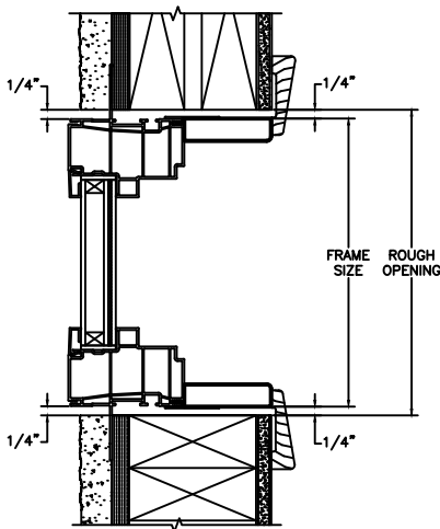
HEAD JAMB & SILL 2 X 4 FRAME WITH STUCCO
