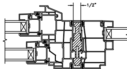
VERTICAL 1/2" MULLION OPERATOR/FIXED
