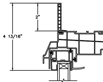
2" FLANGE
