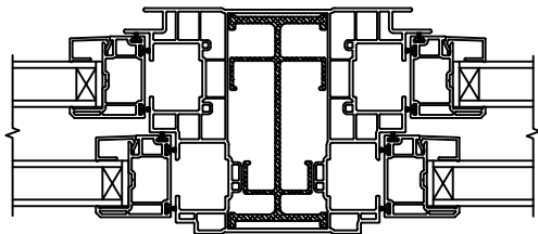
VERTICAL T-BAR OPERATOR/OPERATOR
