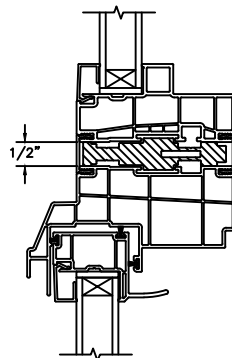
HORIZONTAL 1/2" MULLION RADIUS/OPERATOR
