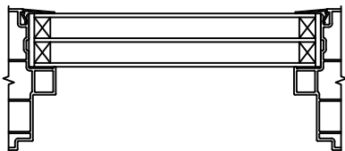
TRIPLE IG INSULATING GLASS
