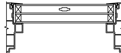
TRIPLE IG 3/4" PROFILED INNERGRILLE
