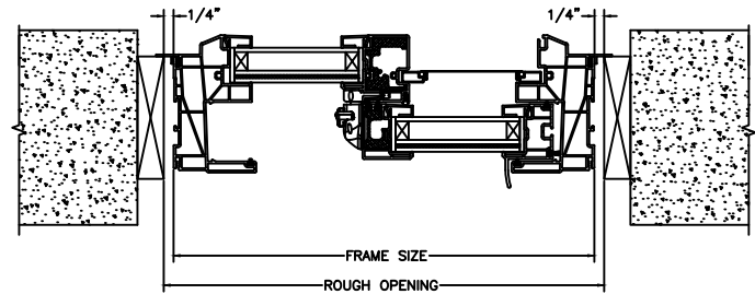
JAMBS BLOCK WALL WITH 1 X 4 1/2" FLANGE OPTION
