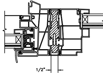
VERTICAL MULLION OPERATOR/FIXED
