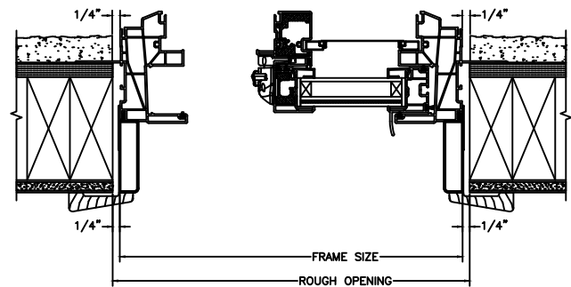
JAMBS 2 X 4 FRAME WITH STUCCO
