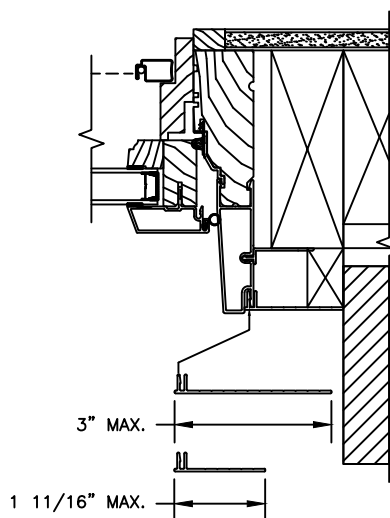
VERTICAL MULLION WITH 2" SPREAD MULL ADDITIONAL WIDTHS INCLUDE: 1", 2", 2 1/2", 3", & 4"
