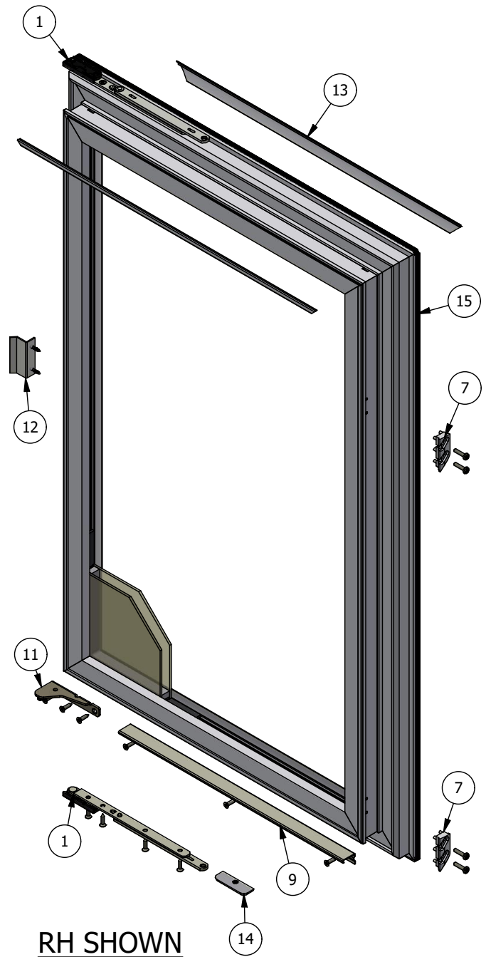
SASH INTERIOR VIEW
