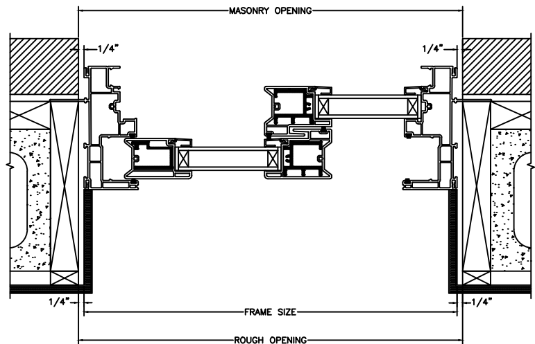
JAMBS 8" CONCRETE BLOCK WALL WITH BRICK VENEER
