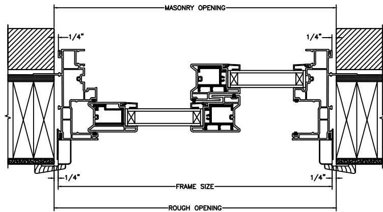
JAMBS 2 X 6 FRAME WITH BRICK VENEER
