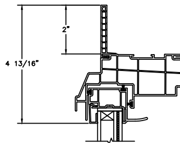
2" FLANGE
