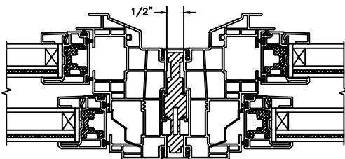
VERTICAL 1/2" MULLION OPERATOR/OPERATOR
