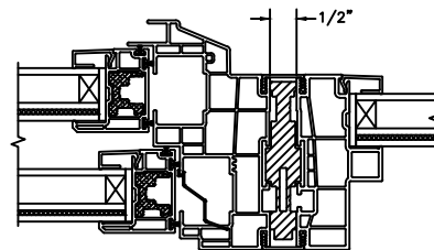
VERTICAL 1/2" MULLION OPERATOR/RADIUS
