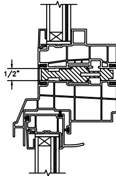
HORIZONTAL 1/2" MULLION RADIUS/OPERATOR
