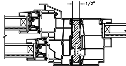
VERTICAL 1/2" MULLION OPERATOR/FIXED
