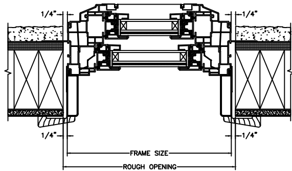
JAMBS 2 X 4 FRAME WITH STUCCO
