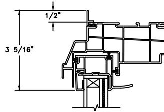
1/2" FLANGE
