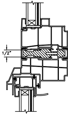
HORIZONTAL 1/2" MULLION FIXED/OPERATOR
