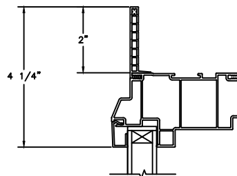
2" FLANGE
