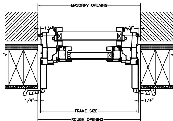
JAMBS 2 X 4 FRAME WITH BRICK VENEER
