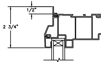
1/2" FLANGE
