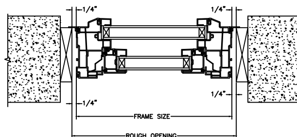
JAMBS BLOCK WALL WITH 1 X 4 1/2" FLANGE OPTION
