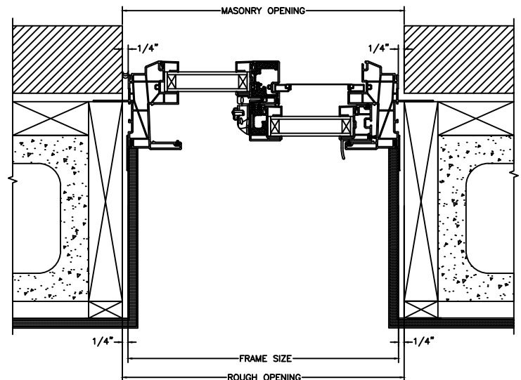
JAMBS 8" CONCRETE BLOCK WALL WITH BRICK VENEER
