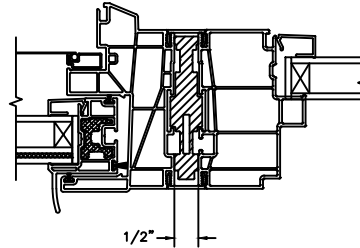
VERTICAL MULLION OPERATOR/FIXED
