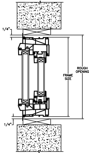
HEAD JAMB & SILL BLOCK WALL WITH 1 X 4 1/2" FLANGE OPTION
