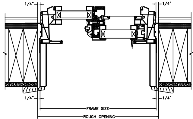
JAMBS 2 X 6 FRAME WITH SIDING
