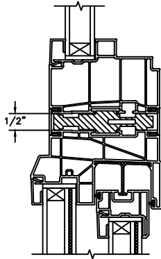
HORIZONTAL MULLION FIXED/OPERATOR
