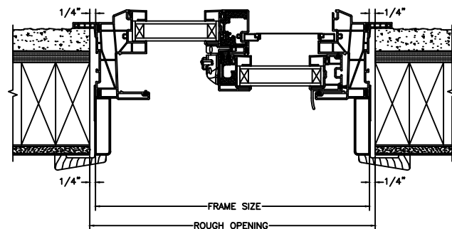
JAMBS 2 X 4 FRAME WITH STUCCO 1" OR 2" FLANGE OPTION
