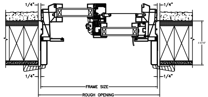
JAMBS 2 X 4 FRAME WITH STUCCO
