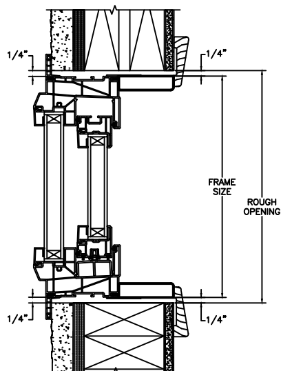
HEAD JAMB & SILL 2 X 4 FRAME WITH STUCCO 1" OR 2" FLANGE OPTION
