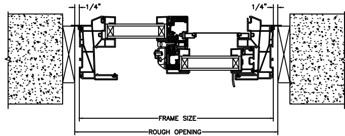
JAMBS BLOCK WALL WITH 1 X 4 1/2" FLANGE OPTION
