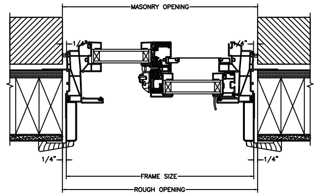
JAMBS 2 X 4 FRAME WITH BRICK VENEER
