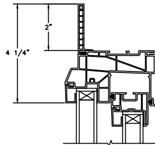
2" FLANGE
