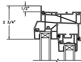
1/2" FLANGE
