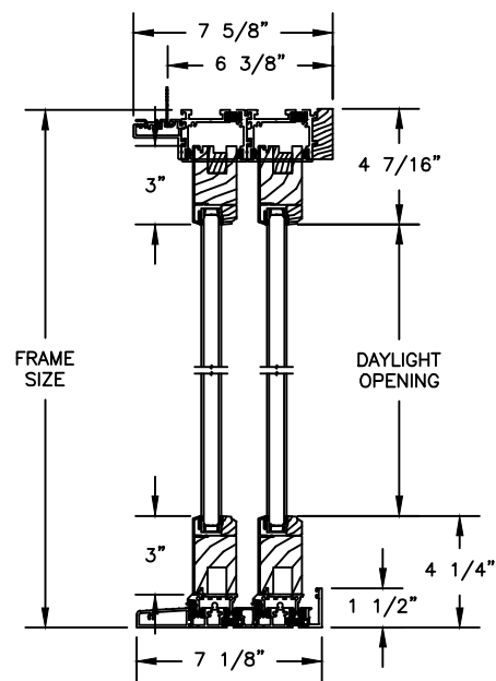
OPERATING HEAD JAMB & FULL SILL
