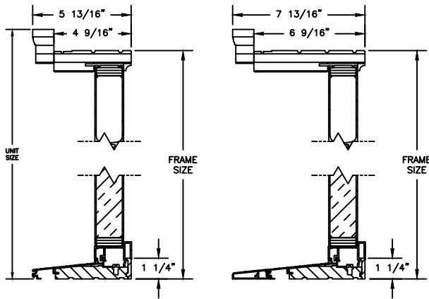
FIXED SIDELITE
