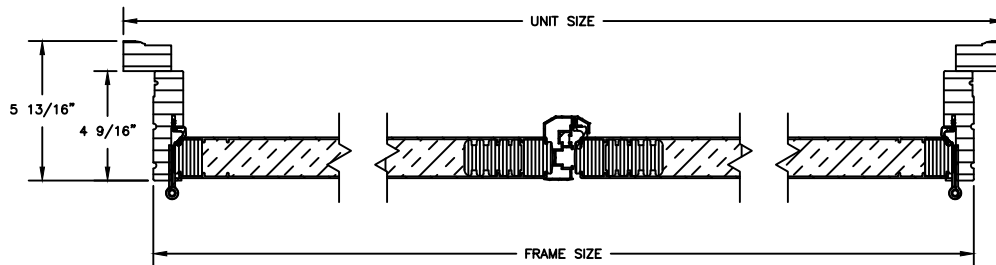
FRENCH INSWING: 4 9/16 JAMB
