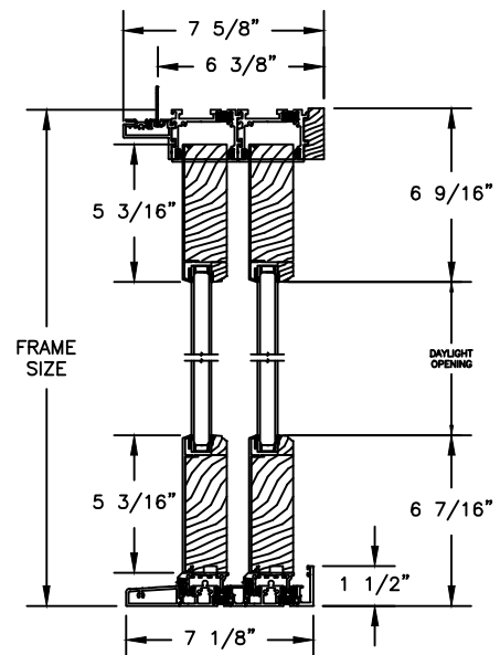
OPERATING HEAD JAMB & FULL SILL
