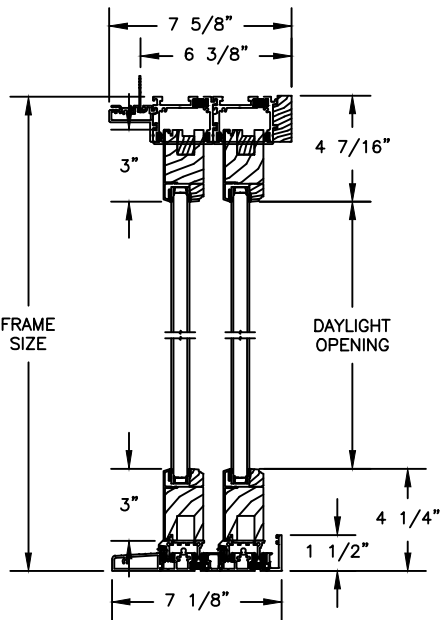
OPERATING HEAD JAMB & FULL SILL
