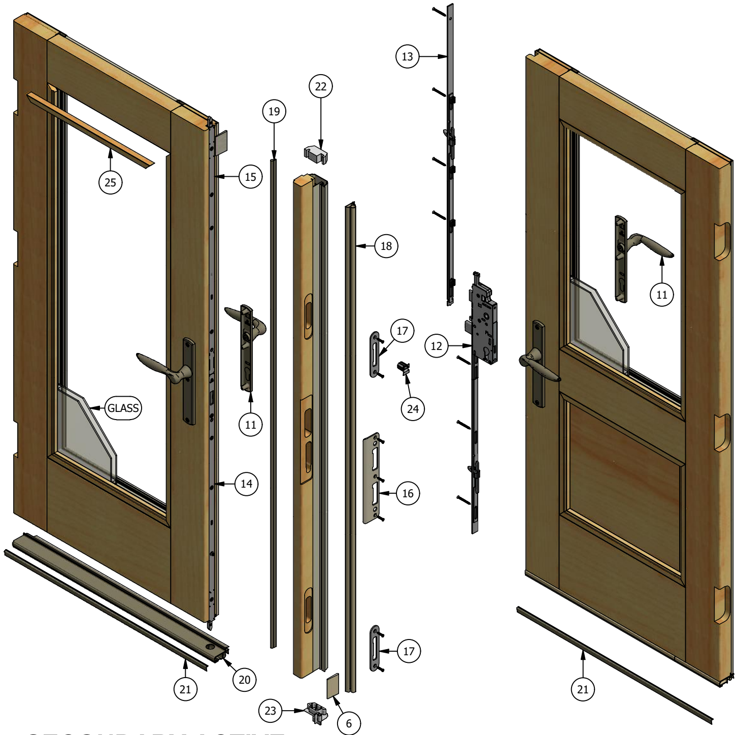
SECONDARY ACTIVE PANEL INTERIOR VIEW
