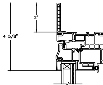
2" FLANGE
