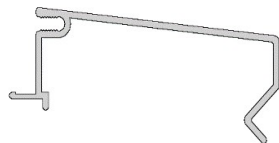
SLIDING PATIO DOOR HEAD & SIDE JAMB COVER
