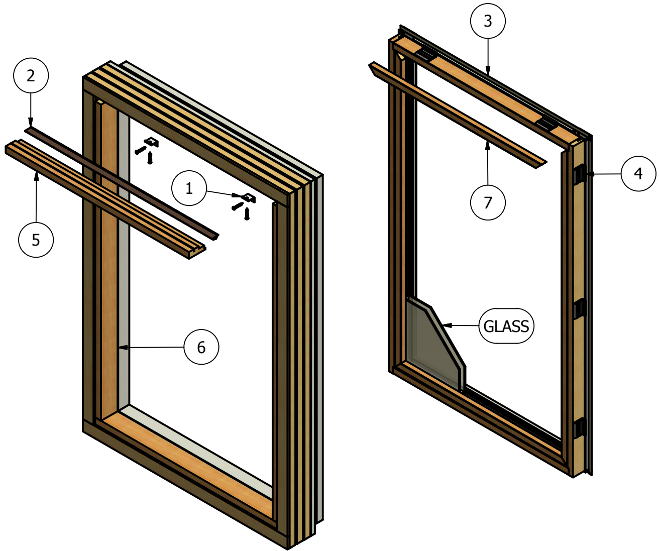
FRAME INTERIOR VIEW
