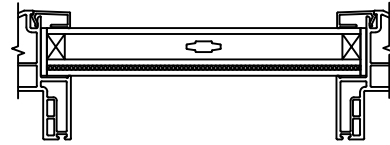
3/4" PROFILED INNERGRILLE
