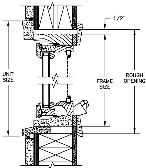
HEAD JAMB & SILL 2 X 4 FRAME WITH STUCCO
