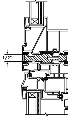
HORIZONTAL MULLION PICTURE/OPERATOR
