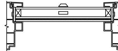
5/8" GRILLE BAR (EXTERIOR ONLY) WITH 5/8" FLAT INNERGRILLE
