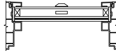
7/8" GRILLE BAR (EXTERIOR ONLY) WITH 13/16" FLAT INNERGRILLE
