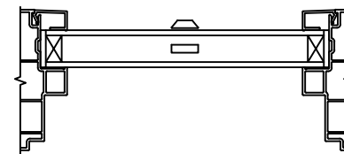
5/8" GRILLE BAR (EXTERIOR ONLY) WITH 5/8" FLAT INNERGRILLE
