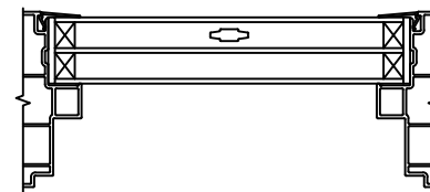
TRIPLE IG 3/4" PROFILED INNERGRILLE
