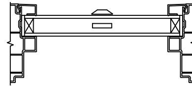
7/8" GRILLE BAR (EXTERIOR ONLY) WITH 13/16" FLAT INNERGRILLE
