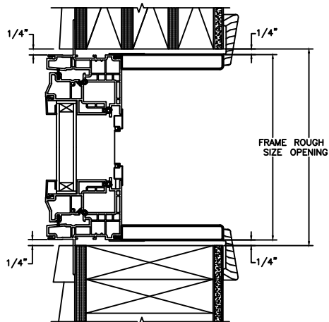
HEAD JAMB & SILL 2 X 6 FRAME WITH SIDING SIDING
