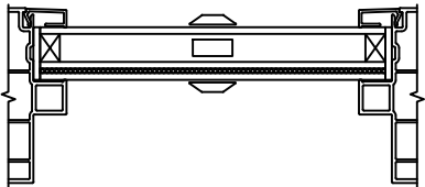
7/8" GRILLE BAR WITH INNERBAR
