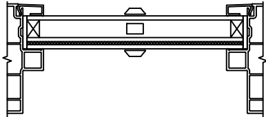
5/8" GRILLE BAR WITH INNERBAR
