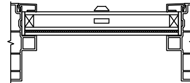
5/8" GRILLE BAR (EXTERIOR ONLY) WITH 5/8" FLAT INNERGRILLE
