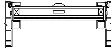
7/8" GRILLE BAR (EXTERIOR ONLY) WITH 13/16" FLAT INNERGRILLE
