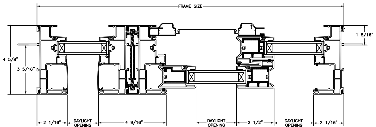
UNIT WITH SIDE LIGHT JAMBS
