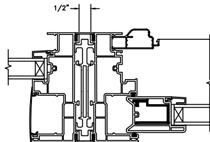
VERTICAL MULLION SIDELITE/OPERATOR
