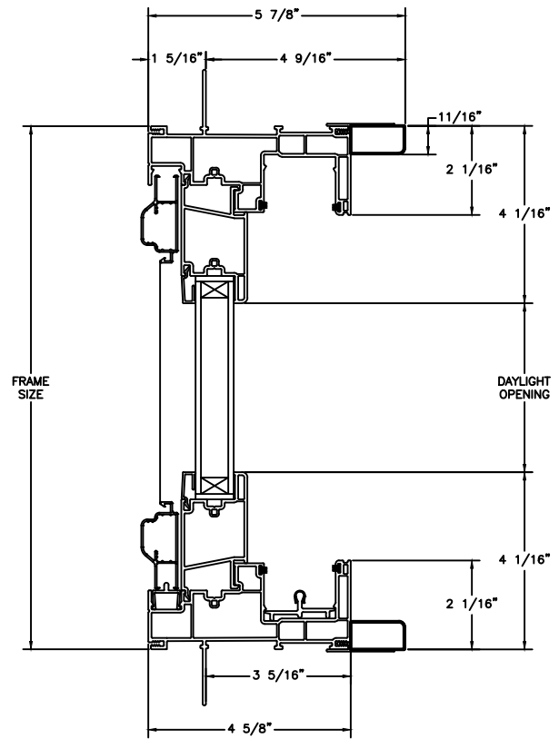
STATIONARY HEAD JAMB & SILL
