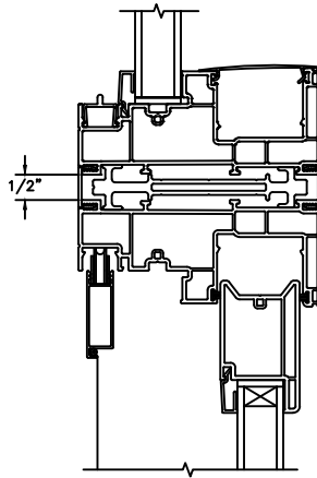
HORIZONTAL MULLION TRANSOM/OPERATOR
