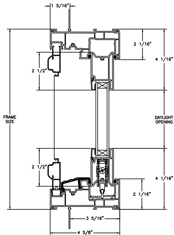
OPERATING HEAD JAMB & SILL
