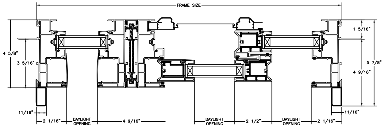
UNIT WITH SIDE LIGHT JAMBS
