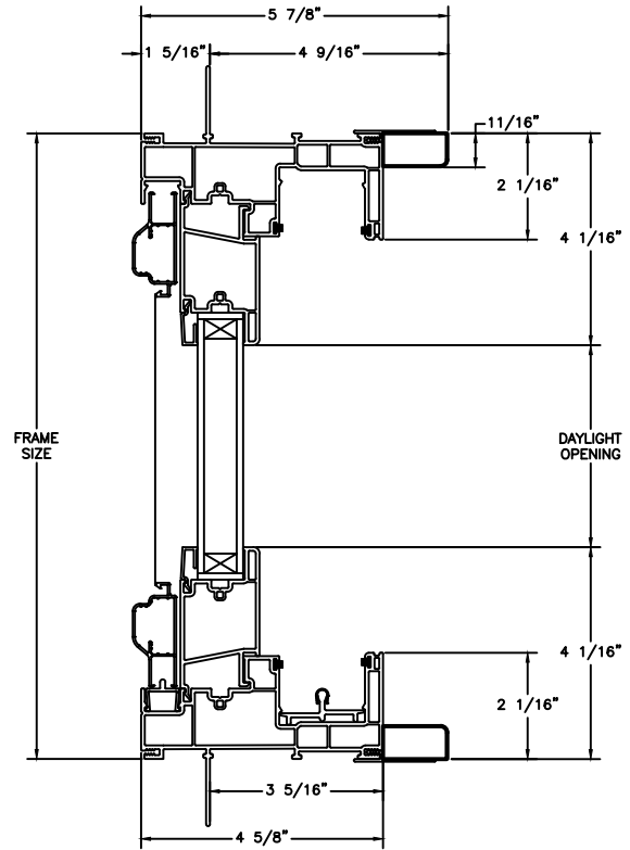
STATIONARY HEAD JAMB & SILL
