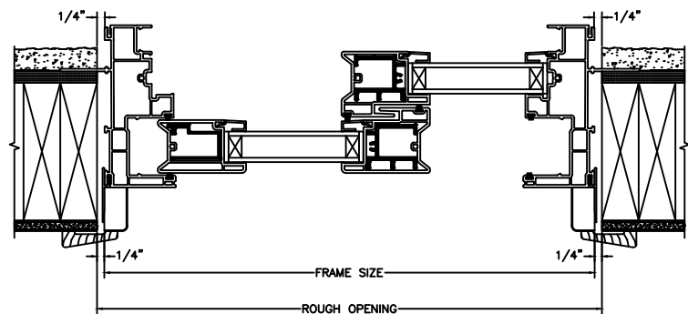
JAMBS 2 X 6 FRAME WITH STUCCO
