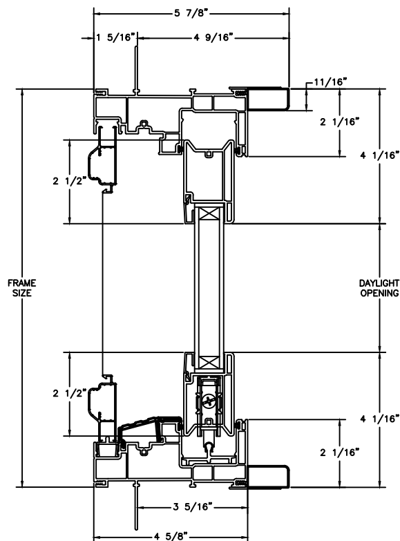
OPERATING HEAD JAMB & SILL
